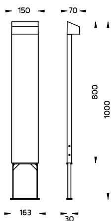
SKUNA – Bollard Slim Base
