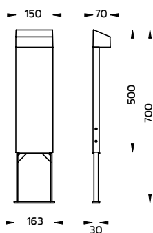
SKUNA – Short Bollard Slim Base
