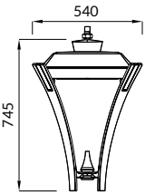
Suspended with aluminium frame
